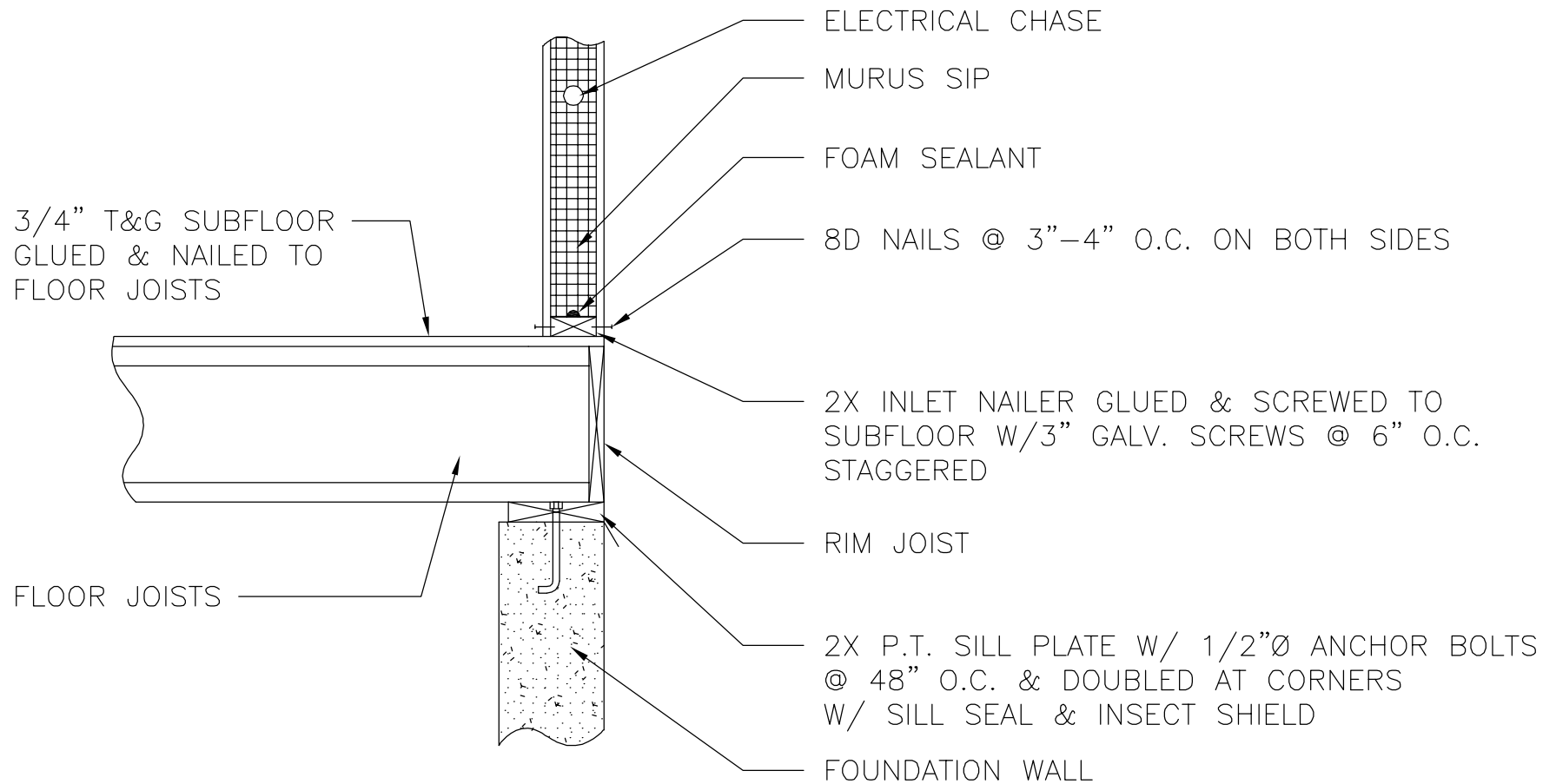
3 PLATFORM FRAMED @ FIRST FLOOR THE MURUS COMPANY
