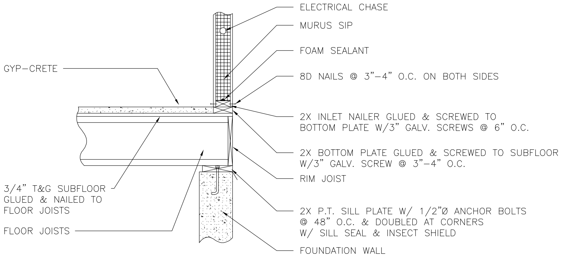
5 GYP-CRETE ON FIRST FLOOR THE MURUS COMPANY
