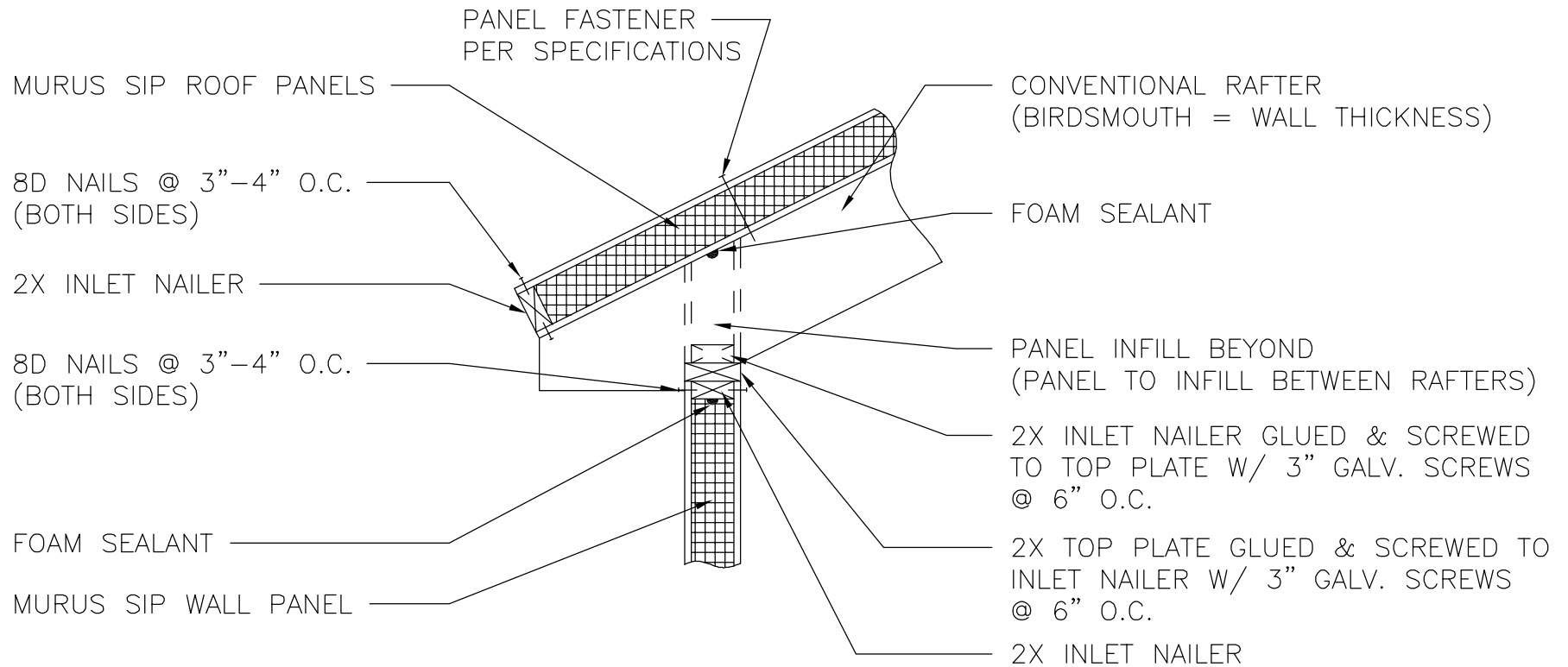
17 ROOF PANELS ON RAFTERS THE MURUS COMPANY
