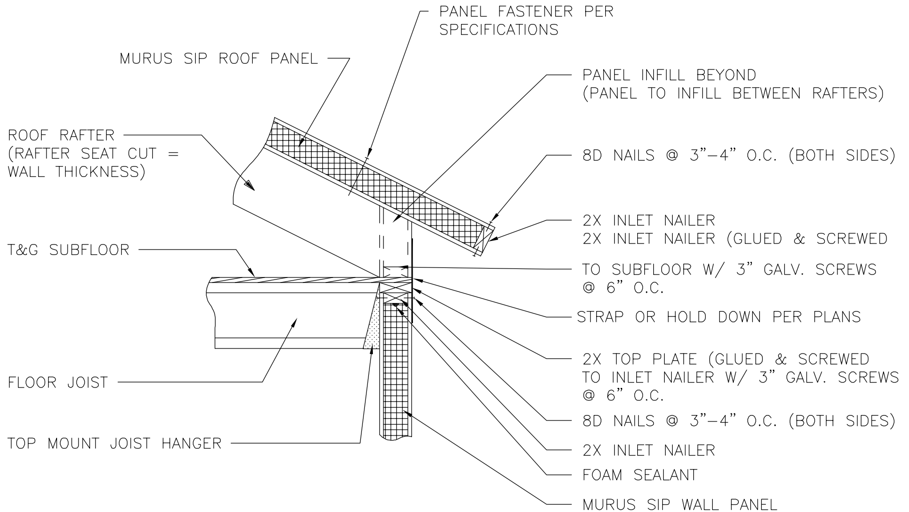
15 RAFTER ON FLOOR SYSTEM THE MURUS COMPANY
