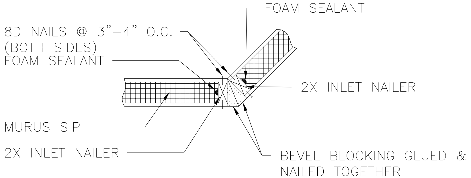
45° CONNECTION DETAIL 8 BEVELED BLOCKING THE MURUS COMPANY
