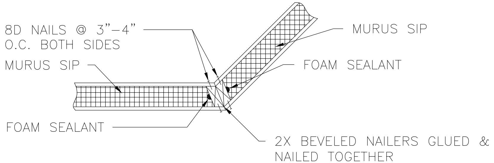
7 45° CONNECTION DETAIL BEVELED PANEL THE MURUS COMPANY
