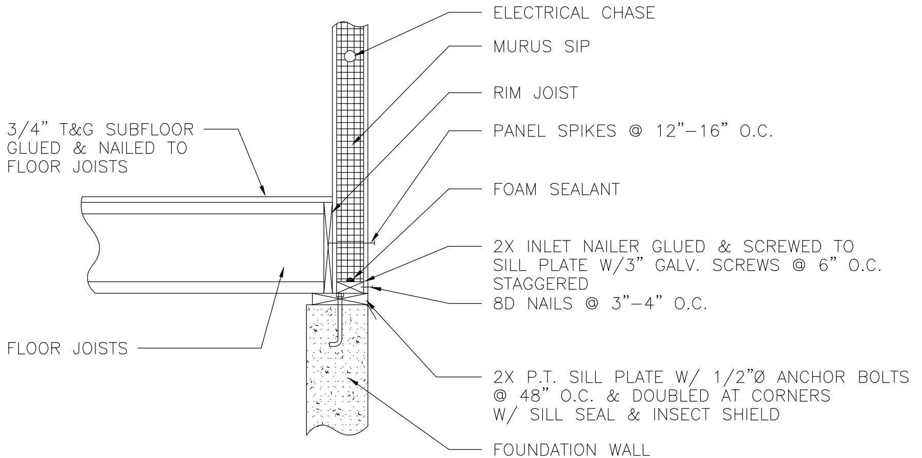
① WRAPPED DECK – FIRST FLOOR THE MURUS COMPANY
